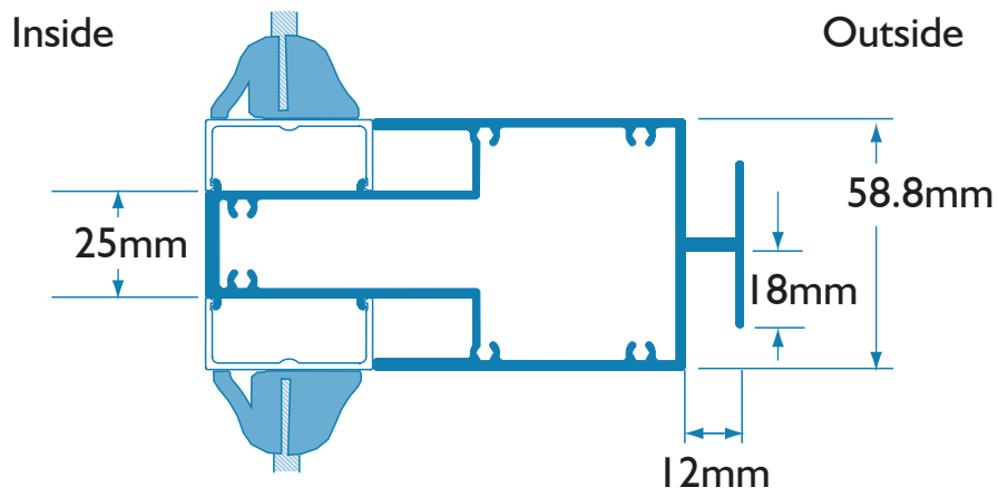
Heavy Duty Mullion
